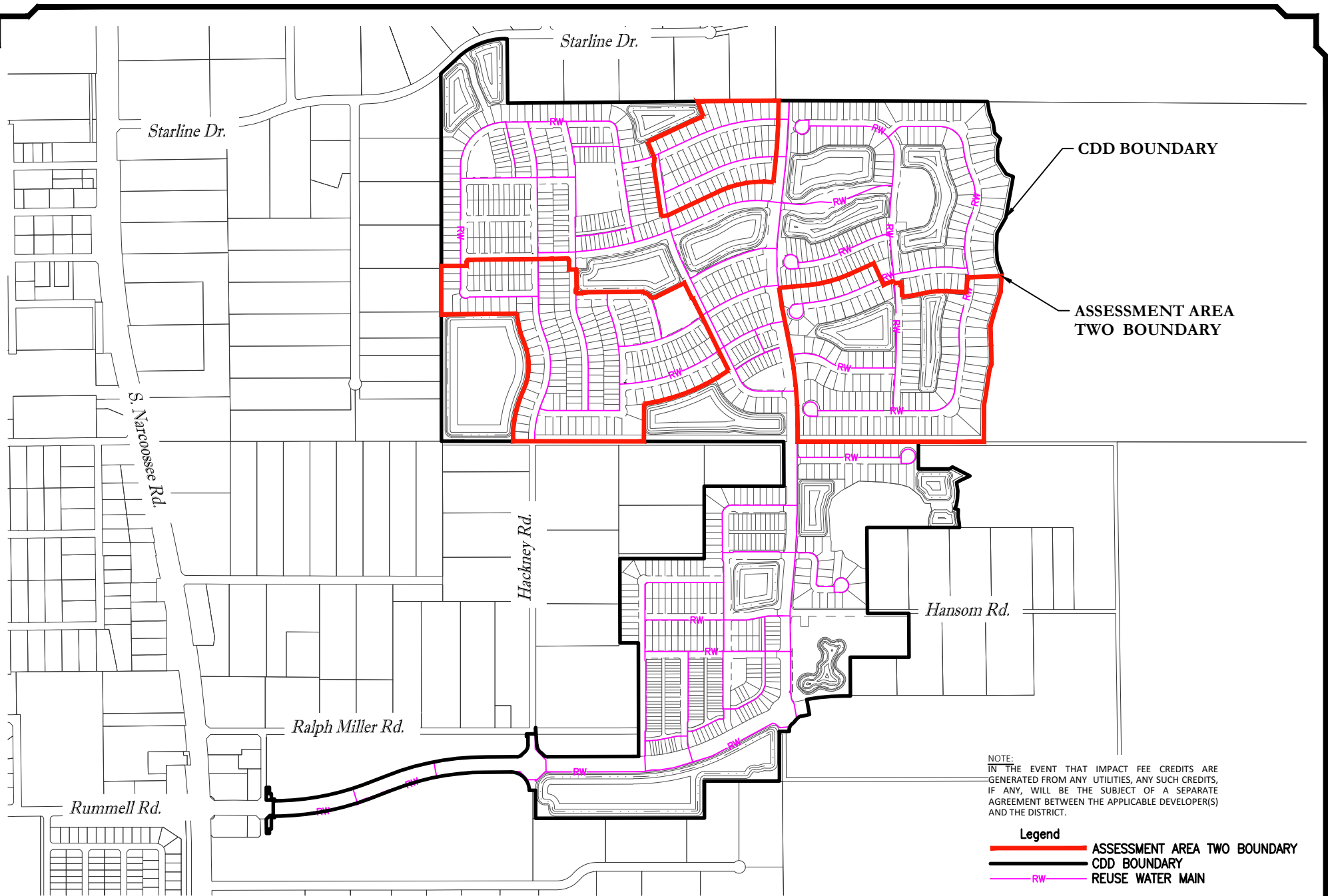
Reuse Water Distribution System Map - Assessment Area Two
