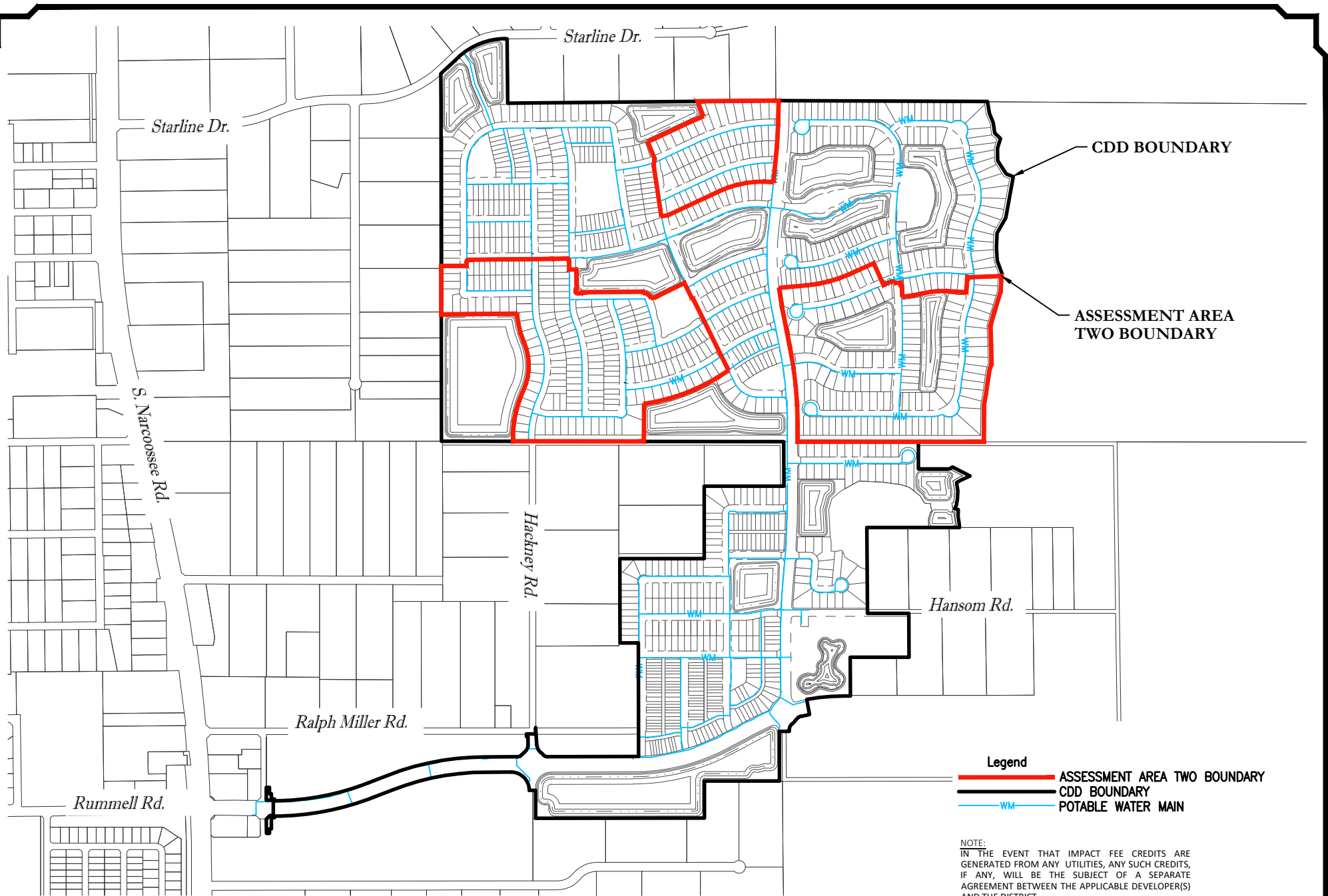
Potable Water Distribution System Map - Assessment Area Two
